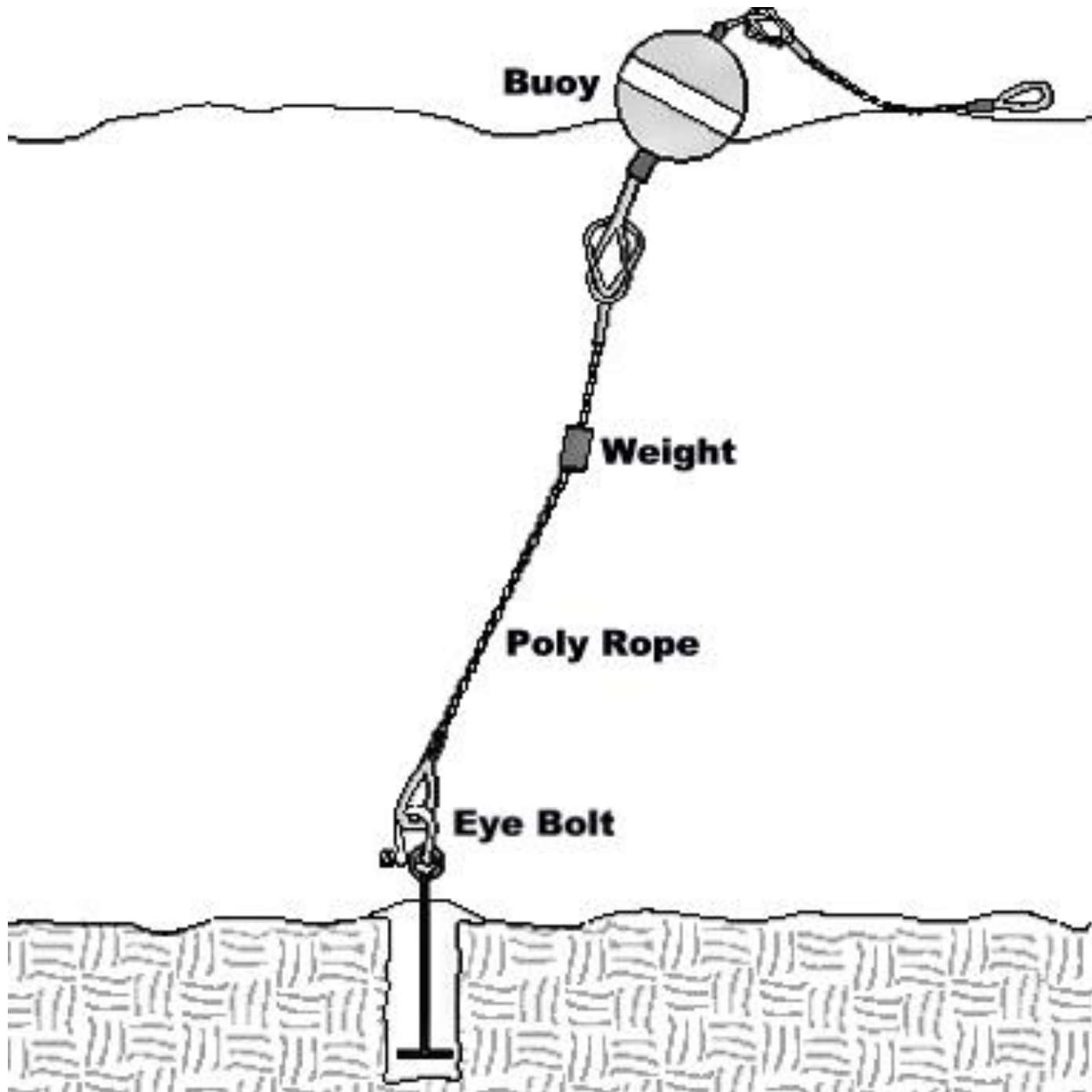
mooring buoy
